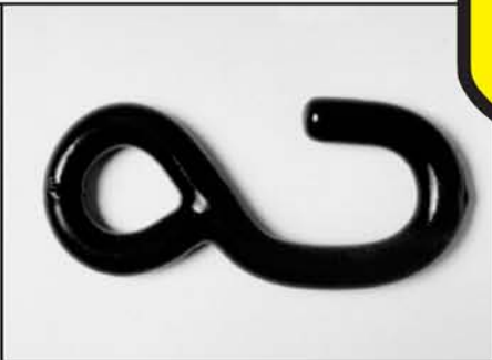
ITEM: Vinyl-coated S-Hook (2) BREAK STRENGTH (lbs.): 1500 W.L.L. (lbs.): 500
