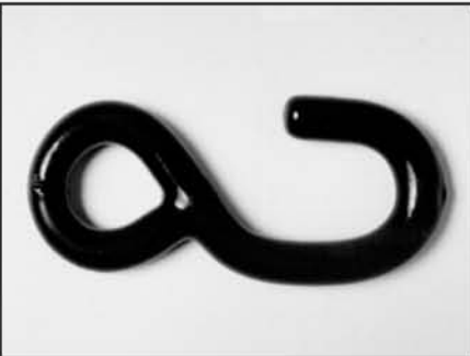
ITEM: Vinyl-coated S-Hook (1) BREAK STRENGTH (lbs.): 2500 W.L.L. (lbs.): 800
